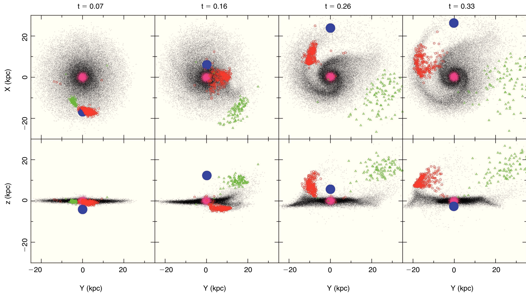
Figure 4 Morphological Evolution of model A. Only disk (black dots) and bulge (grey dots) particles are plotted. Dots enclosed by small triangles (in the case of sub-model A1) or circles (for sub-model A2) and are the particles which settle in the region of Complex C. The solid circle represents the position of the perturber. The rotation axis of the Milky Way is the negative direction of the z axis. The upper panels show the Milky Way as seen from the South Galactic Pole (and hence the disk is rotating counter-clockwise). The units of time shown at the top of the panels are Gyr.
