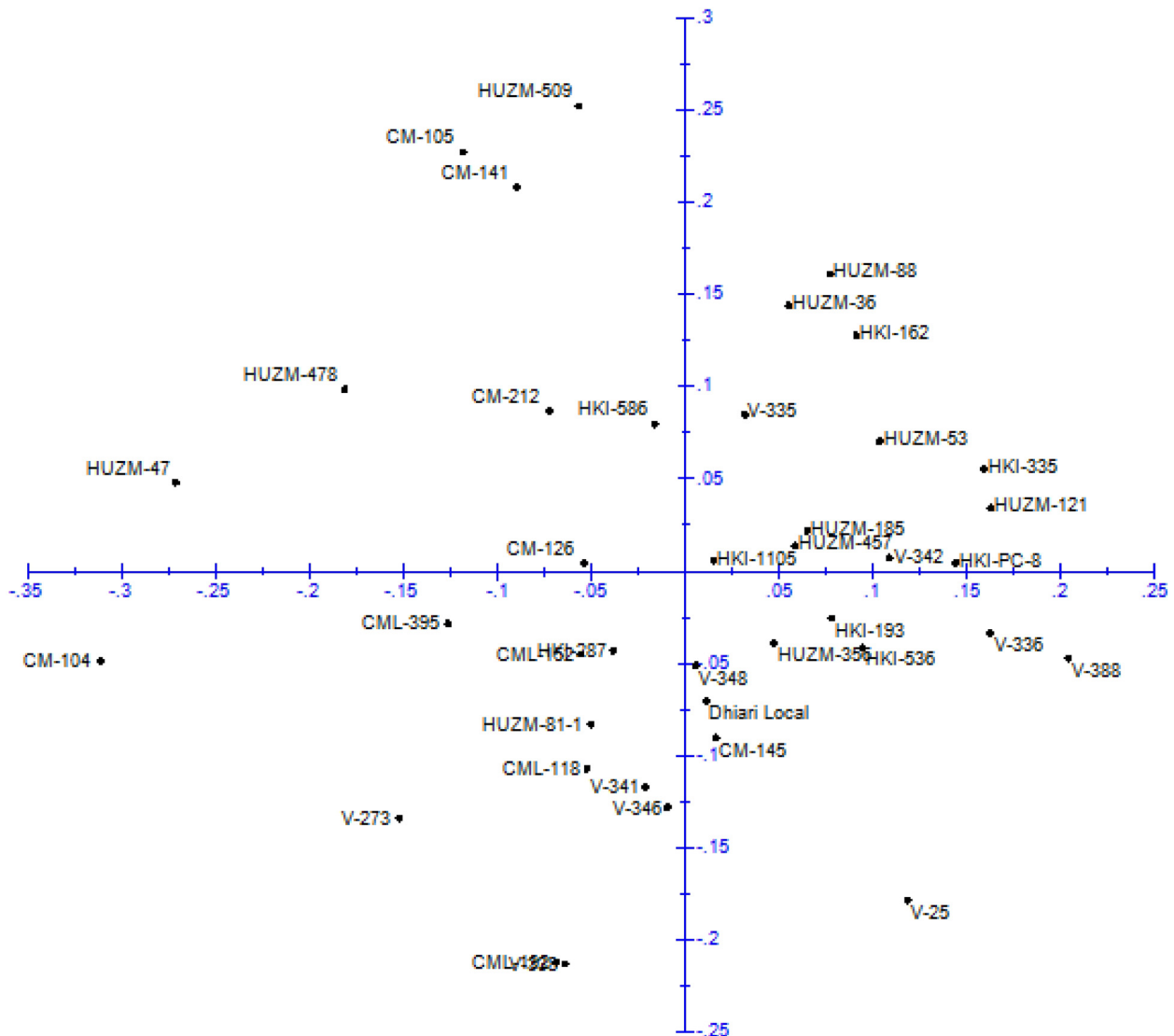
Figure 3. Principal coordinate analysis (PCoA) among 40 maize inbreds using 75 SSR markers.
