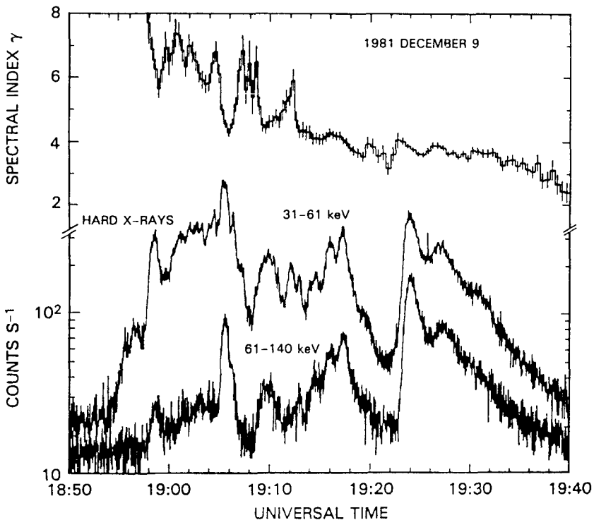
Fig. 7. Hard X-ray time profiles (31–61 keV and 61–140 keV) of the dynamic flare on 9 December, 1981. The uppermost curve shows the gradual decrease of the spectral index \gamma , relatively unaffected by variations in the X-ray flux. (After Cliver et al. , 1986.)
