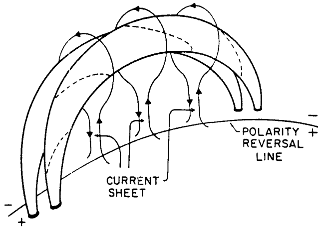
Fig. 10. Schematic representation of the development of an extended current sheet beneath an erupting filament. (After Sturrock et al. , 1984.)
