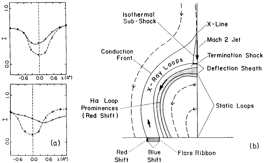
Fig. 3. (a) An example of observed H\alpha line profiles (solid lines) in the ribbons ( above ) and in the loops ( below ) of the dynamic flare of 16 May 1981. Dashed lines show the quiet-Sun reference profile. The blue shift in the ribbons corresponds to an upflow velocity of 4.5 \text{ km s}^{-1} ; the red shift in the loops corresponds to a downflow velocity of 24 \text{ km s}^{-1} for optically thick, and 45 \text{ km s}^{-1} for optically thin loops. (b) The inferred flow pattern for a reconnection model of the gradual phase (see text). (After Schmieder et al. , 1987.)
