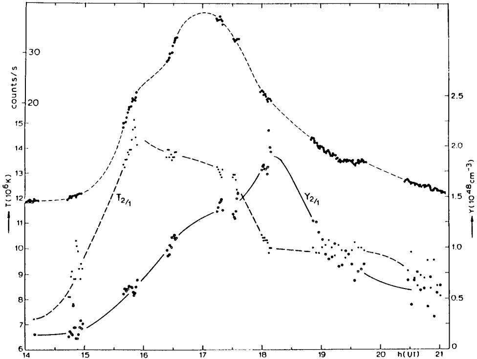
Fig. 5. Time development of the giant post-flare arch that followed the dynamic flare of 14:44 UT on 6 November, 1980 (tentatively the 'arch' of Figure 4). All curves refer to an average altitude of 100 000 km. The upper curve shows the number of counts in 3.5–5.5 keV X-rays, the lower ones the temperature ( T_{2/1} ; left scale) and emission measure ( Y_{2/1} ; right scale). (After Švestka, 1984.)
