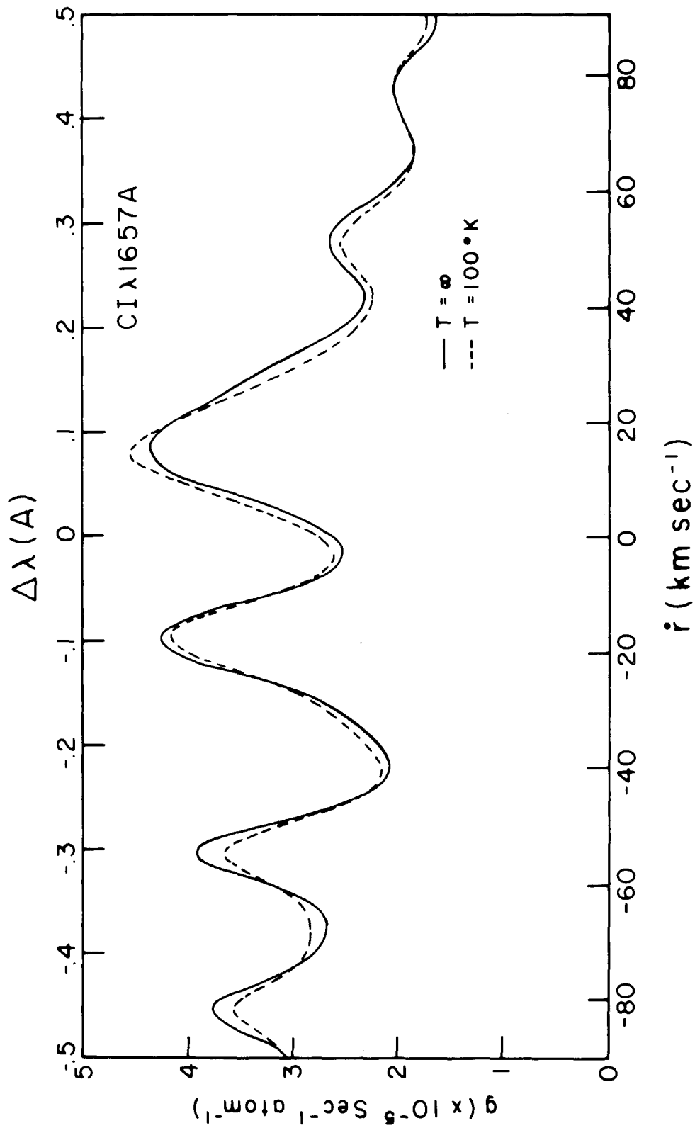
Fig. 2. Dependence of the CI 1657 A g-factor on heliocentric velocity.
