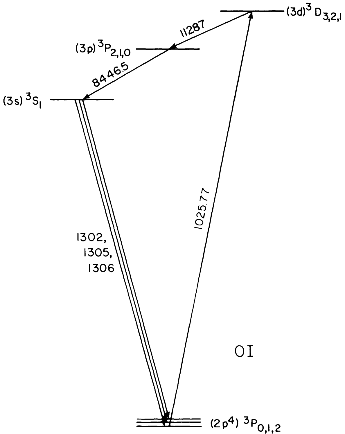
Fig. 5. Fluorescence mechanism for excitation of OI 1302 Å via solar Ly \beta radiation.
