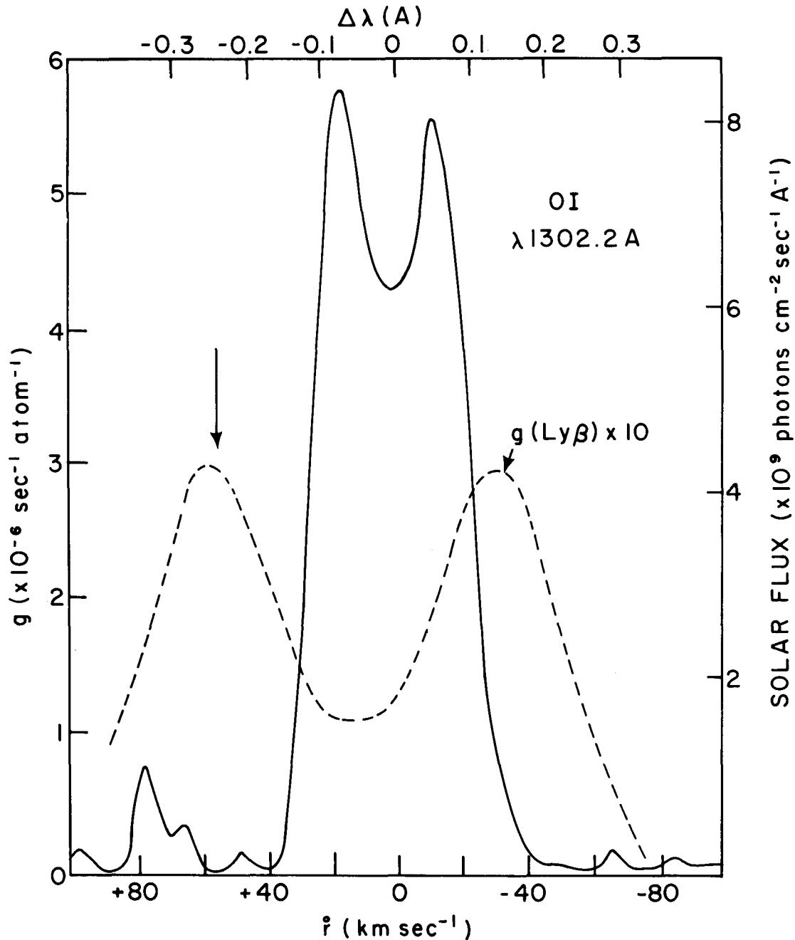
Fig. 4. High resolution profile of the solar O I 1302.2 Å line. The O I g-factor is shown for both resonance scattering and fluorescence excited by solar Ly \beta as a function of heliocentric velocity. The arrows correspond to the observations of Feldman et al. (1974) and Opal et al. (1974).
