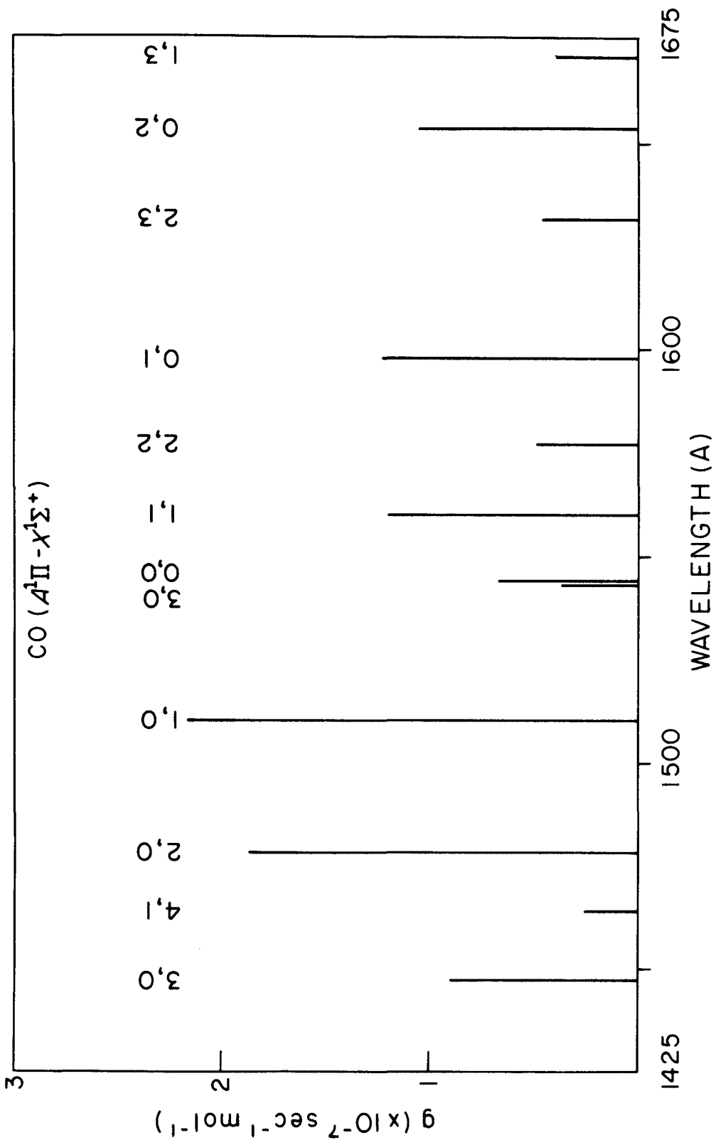
Fig. 7. g-factors for the strongest bands of the CO fourth positive system.
