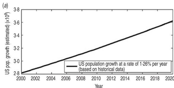
Fig. 3. Baseline model projections: potential MRSA infection incidence increase and gradual replacement of MSSA over the next decade in the USA in the absence of systematic infection control, based on the 1999–2005 national trends (infection and colonization) and assuming strong competition between MRSA and MSSA for colonization of susceptible hosts [19]. (a) Projection of US population growth for period 2000–2020, based on historical US Census data.
