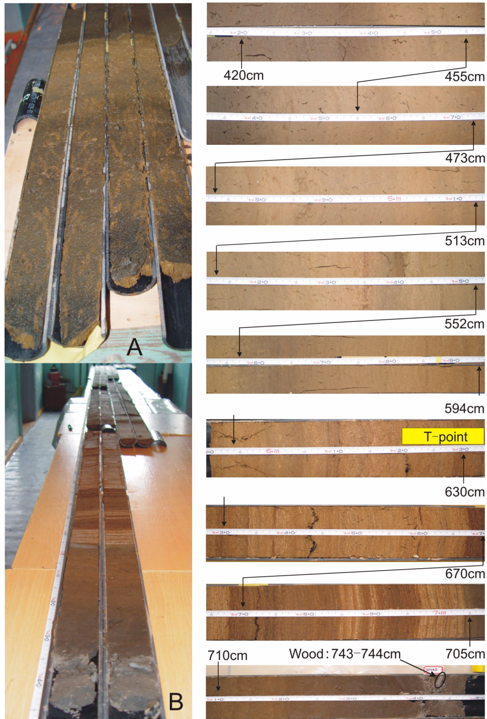
Figure 2 A detailed picture of the core stratigraphy, left column: fresh cores viewed from the top (A) and from the bottom (B); right column, the core from ~4.2 m to the bottom (T-point marks the reverse point of AMS ^{14}\text{C} ages; see also Figures 3 and 4).
