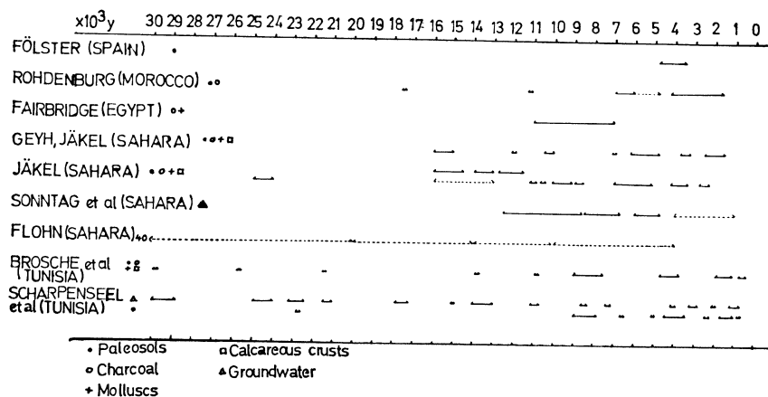
Fig 3. Age spans covered by radiocarbon dates
