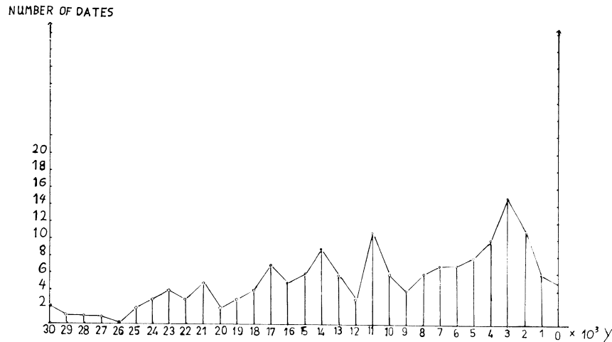
Fig 2. Histogram of groundwater dates (Tunisia) number of dates each full thousand \pm 0.5 thousand years
