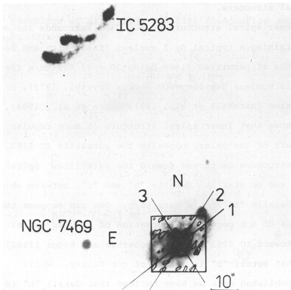
Figure 2. Radio isophotes of central region of NGC 7469 at 6 cm according to Ulvestadt et al. (1981) projected on the photo of the galaxy. 1,2,3 - directions of radio isophotes stretching.
