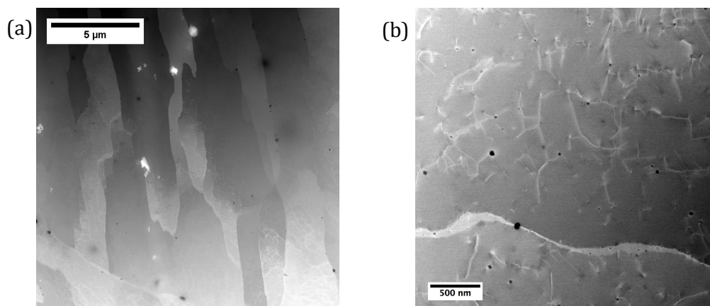
Figure 2: (a) High-angle annular dark field (HAADF) micrograph showing the columnar grains of AM 316L stainless steel, (b) Medium-angle annular dark field (MAADF) micrograph showing high number density of dislocations present in a grain of AM 316L stainless steel. The line features with brighter contrast are dislocations. Ti-rich oxides that appear in darker contrast are clearly visible and are decorated along grain boundary or associated with dislocation lines.
