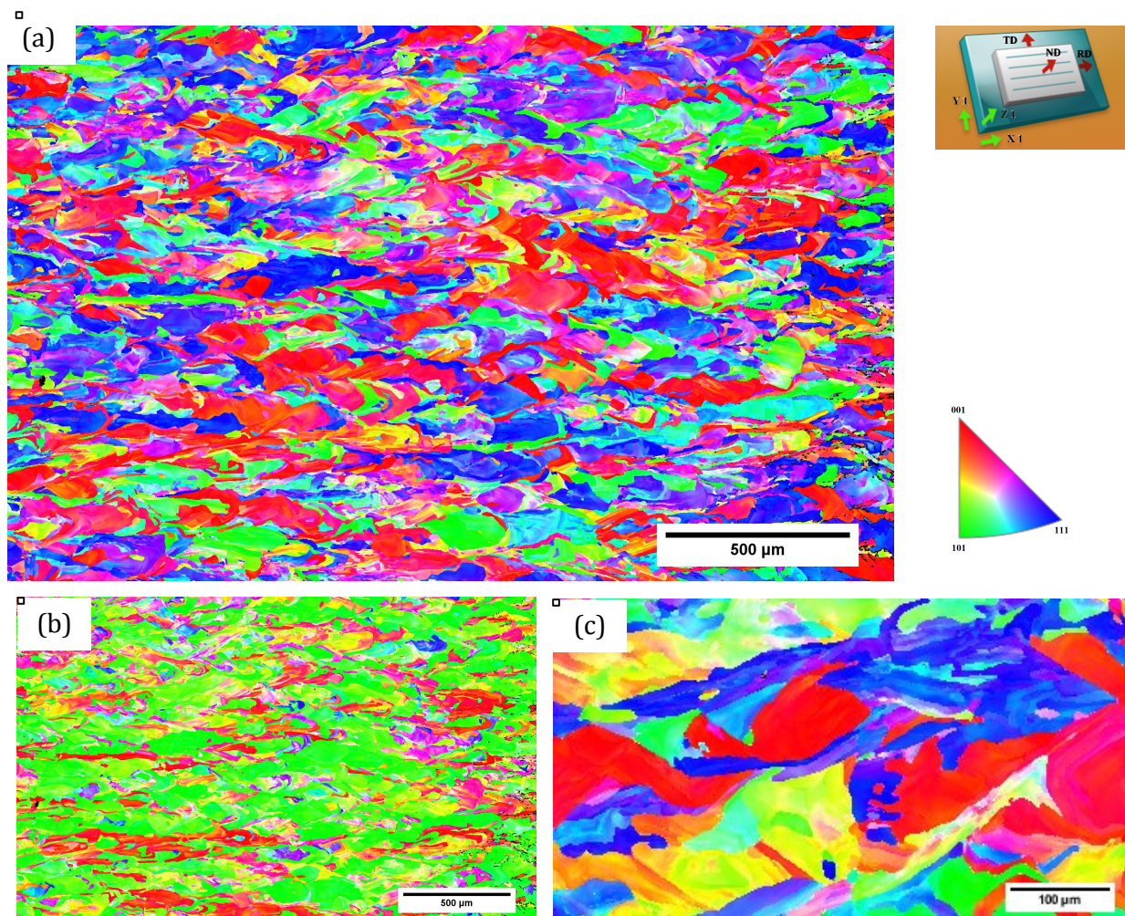
Figure 1: EBSD grains orientation maps showing (a) grain orientation at direction of IPF-Z, (b) grain orientation along the deposition/melting direction, i.e. IPF-X or RD, & (c) higher magnification of grain orientation along the direction of IPF Z
