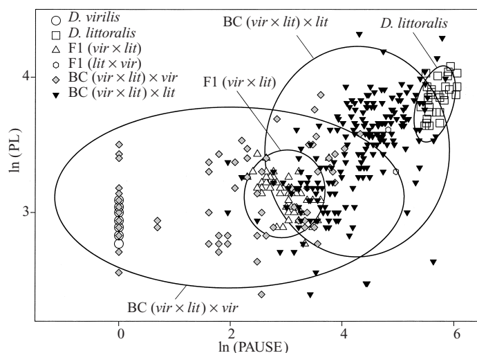
Fig. 2. Bivariate scattergrams and 90% equal-frequency ellipses of pulse and pause lengths (logarithms) of D. virilis and D. littoralis strains and interspecific F1 and backcross (BC) hybrids. Ellipses could not be drawn for D. virilis , because in this species the sound pulses follow each other without a pause, or for D. littoralis × D. virilis hybrids, because of the scarcity of the data points.
