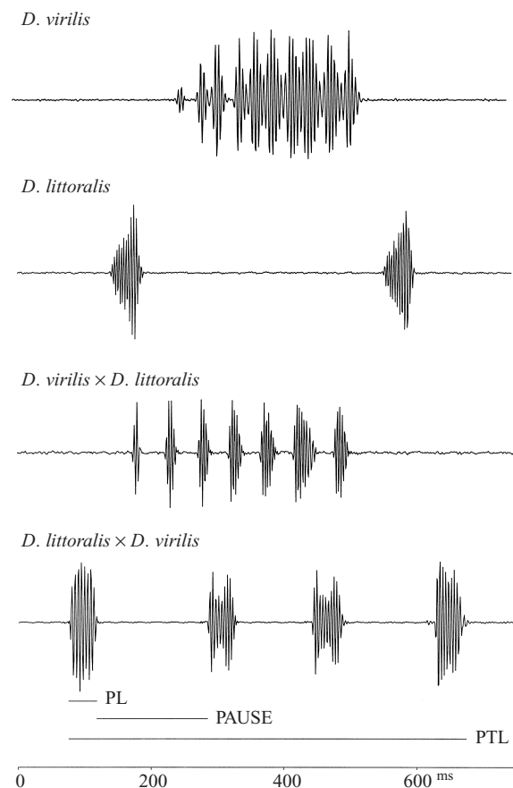
Fig. 1. Oscillograms of the male courtship songs of D. virilis , D. littoralis and the reciprocal F1 hybrids having the X chromosome of D. virilis ( D. virilis × D. littoralis ) or D. littoralis ( D. littoralis × D. virilis ).
