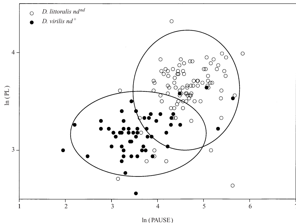
Fig. 3. Bivariate scattergrams and 90% equal-frequency ellipses of pulse and pause lengths of ( D. virilis × D. littoralis ) × D. littoralis backcross hybrids expressing/not expressing an X chromosomal marker gene, nd , of D. littoralis .
