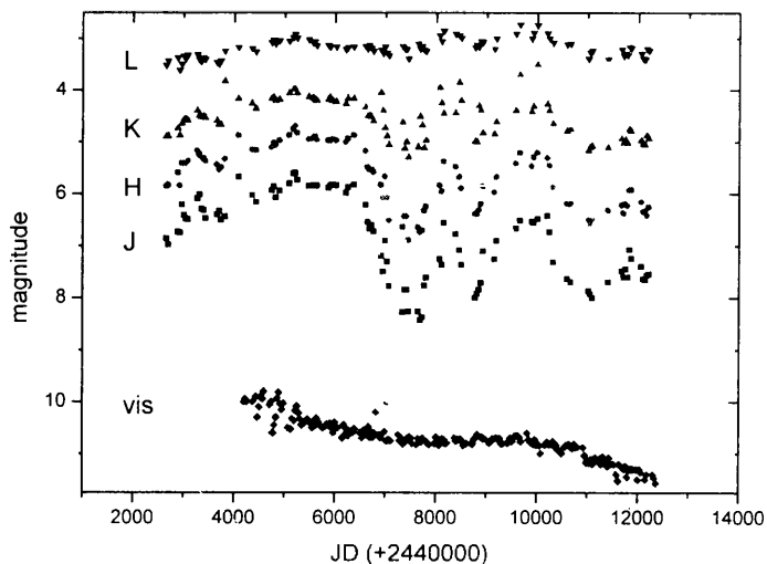
Fig. 1. JHKL light curves corrected for mira pulsations and the visual light curve over about 25 years
