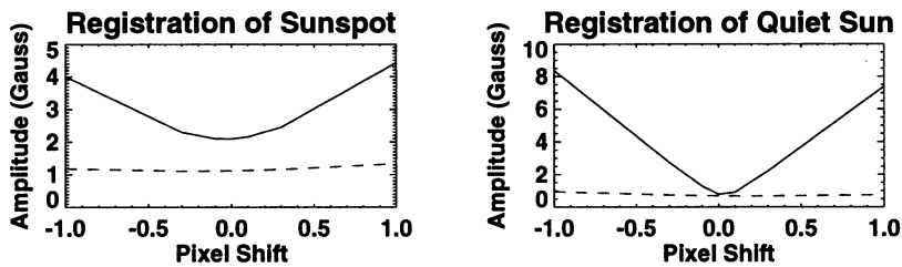
Figure 3. LCP and RCP images are shifted against each other to generate misregistered datasets. Resulting B signal (solid) and noise (dashed) amplitude are plotted vs N-S misregistration for sunspot (left) and quiet sun (right).
