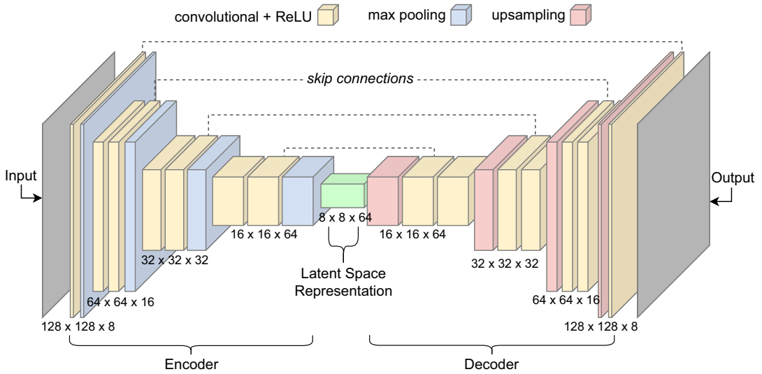
Figure 10. The denoising autoencoder network architecture.
