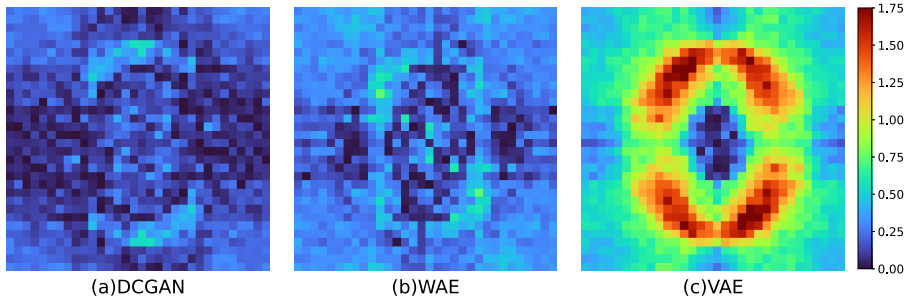
Figure 6. The difference between real geodetic noise and synthesized noise in terms of FFT magnitude spectra.
