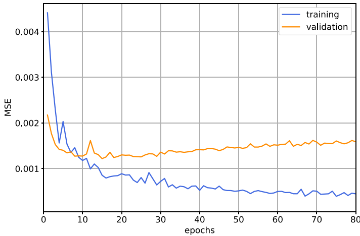
Figure 11. The training and validation curves from the CDAE network trained in Section 4.
