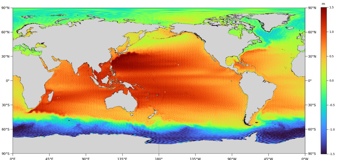
Figure 2. DTU18-EIGEN-6C4 MDT, expanded up to degree/order 280.
