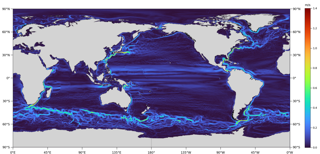
Figure 1. Surface geostrophic current velocity map computed from the high-resolution CMCC-CM2-HR4 climate model (Scoccimarro et al., 2019) prepared for Coupled Model Intercomparison Project Phase 6 (CMIP6).
