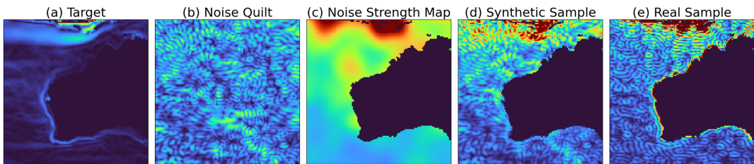
Figure 9. A demonstration of the noise application showing (a) a target training sample from the HadGEM3-GC31-MM climate model; (b) a random noise quilt; (c) the associated noise strength map generated from the smoothed prior MDT; (d) the resulting synthetic sample in which the noise quilt has been applied to the target according to Equation 4 (with k=1.5 ); and (e) a real sample of surface geostrophic currents computed from the DTU18_EIGEN-6C4 geodetic MDT.
