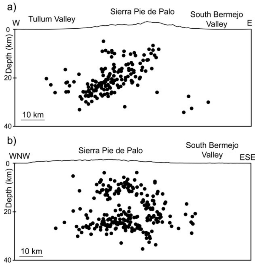
Figure 4. Seismicity profiles below the Sierra Pie de Palo showing seismic foci in vertical cross-sections redrawn after Regnier et al. (1992), (a) for the northern half of the sierra and (b) for the southern half of the sierra. See Regnier et al. (1992) for the original data and precise location of the earthquakes that were projected on the sections. See Figure 3 for location of the cross-sections.
