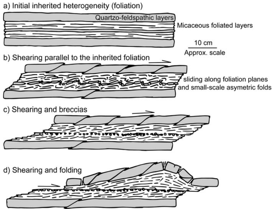
Figure 12. Conceptual model of shear zone development. (a) Inherited metamorphic foliation with both quartzo-feldspathic and mica-rich layers. (b) Shearing induces disharmony with folding of thin quartzo-feldspathic layers embedded between mica-rich layers that most likely accommodate foliation-parallel shear. Layer-parallel shortening of the upper quartzo-feldspathic layer is represented for balancing purposes, although this has not been clearly observed in the field. (c) Breccias resulting from the breakdown of the folded quartzo-feldspathic layer. The shearing localizes in this brecciated zone. (d) Ultimately, this brecciated layer may evolve as a new local décollement allowing the development of larger folds affecting the upper quartzo-feldspathic layers.
