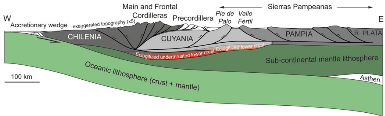
Figure 15. (Colour online) Lithospheric-scale section of the Andes modified from Cristallini and Ramos (2000) (see Fig. 1a for location). The crustal structure at Pie de Palo and below the Precordillera were modified according to the present study. The Moho and lower crustal structure (eclogitized root) are from Ammirati et al. (2013) and Ammirati, Alvarado & Beck (2015). The Eastern Sierras Pampeanas structure is from Ramos et al. (2002) and Perarnau et al. (2012).
