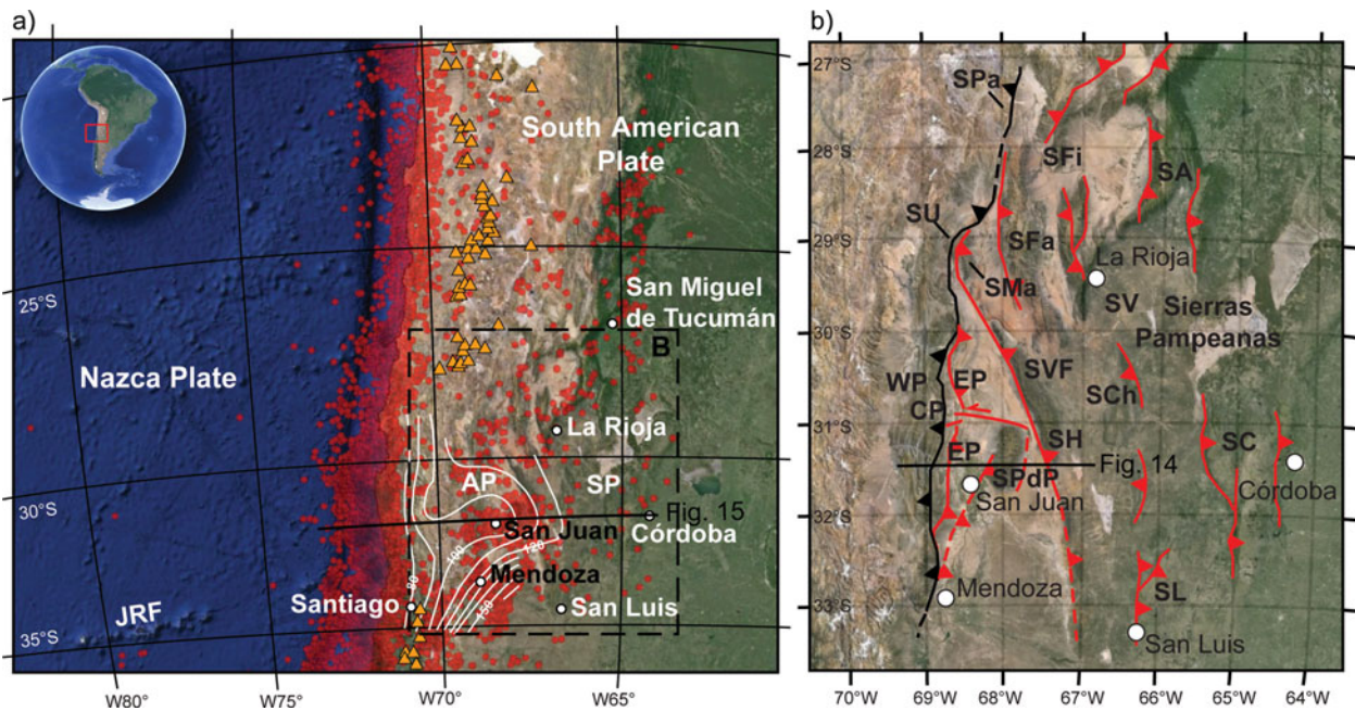
Figure 1. (Colour online) (a) Map of Central Andes (Landsat images and General Bathymetric Charts of the Oceans) together with distribution of active volcanoes (orange solid triangles, Smithsonian Institution, Global Volcanism Program) and seismicity (red solid dots, US Geological Survey seismicity catalogue, M \geq 4.0 and depth \leq 70 km). White solid lines (labelled in km) are isodepths of the Wadati–Benioff plane and highlight the Pampean flat slab of the Nazca plate (after Ammirati et al. 2013). Key: AP, Argentine Precordillera; SP, Sierras Pampeanas; JRF, Juan Fernandez Ridge. (b) Schematic regional structural map of the Sierras Pampeanas. Red solid lines denote active structures. Key: AP, Argentine Precordillera; WP, Western Argentine Precordillera; CP, Central Argentine Precordillera; EP, Eastern Central Precordillera; SPdP, Sierra Pie de Palo; SH, Sierra de la Huerta; SVF, Sierra de Valle Fértil; SMa, Sierra La Maz; SFa, Sierra de Famatina; SFi, Sierra Fiambala; SA, Sierra Ambato; SV, Sierra Velasco; SCh, Sierra Chepes; SC, Sierra de Córdoba; SL, Sierra San Luis; SU, Sierra Umango; SPa, Sierra de las Planchadas.
