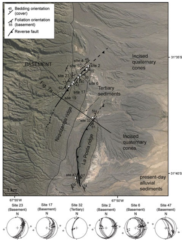
Figure 5. (Colour online) Structural data at Niquizanga. See Figure 3 for location. This area consists mainly of two basement ridges due to W-verging thrust faults affecting both the basement and the Cenozoic sedimentary cover. The faults are NNE–SSW and attest for an ENE–WSW shortening according to the microtectonic data. The kinematic data show axes of deformation in the basement consistent with those in the cover. Fold axes (black dots in the stereonets) are also consistent with an ENE–WSW shortening, both in the basement and the cover. In the investigated sites (white circles with numbers), the basement foliation dips eastward.
