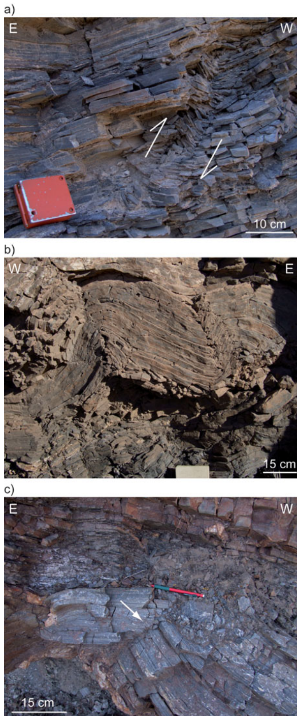
Figure 8. (Colour online) Field photographs of folds affecting the basement rocks. The folds display very brittle style with (a) kink geometries (site 2, Fig. 5), and (b), (c) sharp, fractured hinges with planar limbs (sites 10 and 17, respectively, Fig. 5), while the inherited ductile deformation can still be observed as boudins (c). Note that the fold axes are approximately N–S and that preferential vergence of the folds is systematically a W-vergence.
