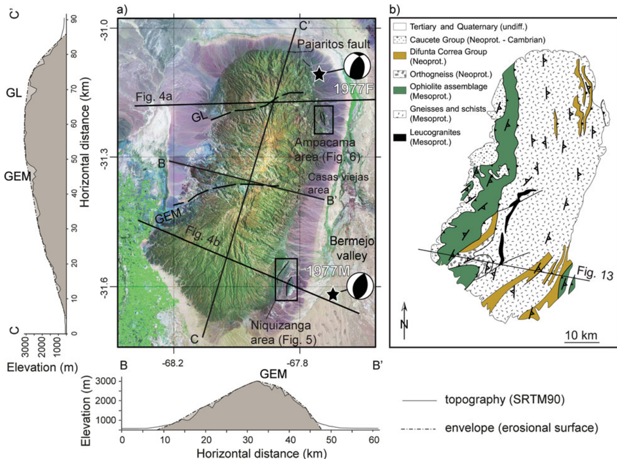
Figure 3. (Colour online) (a) Landsat image of the Sierra Pie de Palo. Both \approx E–W (B–B') and \approx N–S (C–C') topographic cross-sections have been extracted from the Shuttle Radar Topography Mission 1990 digital elevation model (SRTM90 DEM) (thick solid lines). The reconstructed regional erosion surface (thick dotted lines) is after Siame et al. (2015). The two stars locate the two 1977 earthquakes with their respective focal solutions (F for fore shock and M for main shock) (Langer & Hartzell, 1996). Key: GEM, Grande El Molle lineament; GL, Guayaupa–Lima lineament. (b) Geological map with main foliation orientations modified from Ramos and Vujovich (2000), Mulcahy et al. (2011) and Van Staal et al. (2011).
