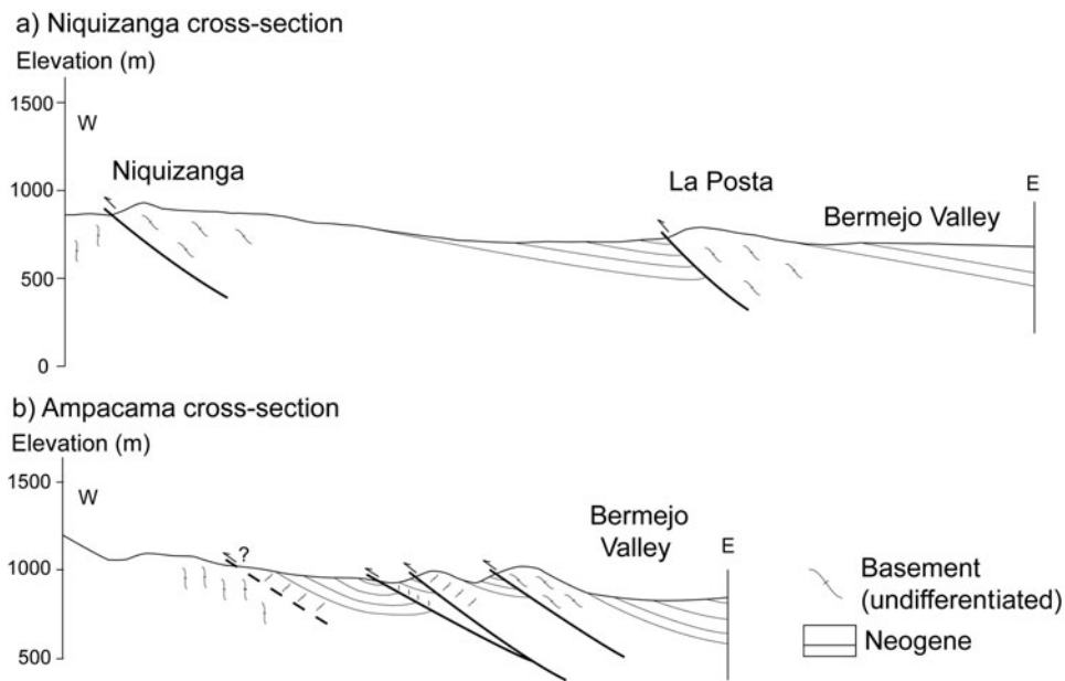
Figure 7. Cross-sections through both investigated areas. See Figures 5 and 6 for location. (a) Cross-section through Niquizanga area. Two faults are mapped and dip about 40^{\circ} E, with Neogene sediments between them. The faults are parallel to the inherited foliation in the basement. (b) Cross-section through Ampacama area. Three main thrusts are represented with dips about 30^{\circ} E. Along one of the faults, the fault plane is parallel to the basement foliation, while elsewhere it is strongly oblique. Between the basement thrust, the Neogene sediments mainly dip about 30^{\circ} E. A fourth fault is suspected in the western part, but no Tertiary sediments crop out to confirm it.
