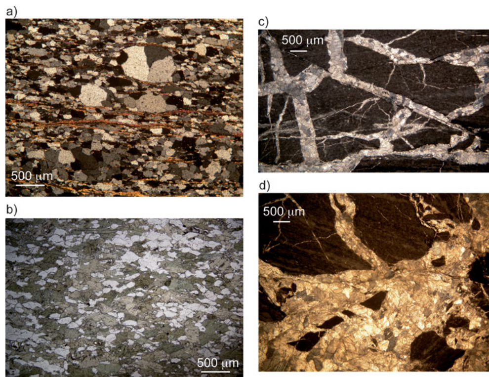
Figure 11. (Colour online) Microphotographs. (a) Micaschist (site 4, Fig. 5) with foliation underlined by quartz and micas. (b) Quartzofeldspathic rocks with a high amount of chlorite and no clear anisotropy (site 96, Fig. 6). (c, d) Breccias and calcitic cement in the brecciated layers (site 23, Fig. 5).
