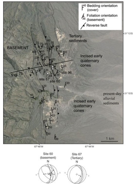
Figure 6. (Colour online) Structural data at Ampacama. See Figure 3 for location. This area consists of two main basement ridges due to W-verging thrust faults in the basement, thrusting above the Cenozoic sediments. The faults are NNW–SSE and attest for an E–W shortening according to the microtectonic data. The kinematic data show axes of deformation in the basement consistent with those in the cover. In the investigated sites (white circles with numbers), the basement foliation usually dips eastward, although in several places it is either vertical or west-dipping.
