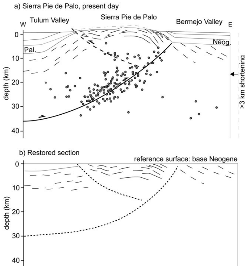
Figure 13. (a) Cross-section of the Pie de Palo (see Fig. 3 for location) and (b) its restoration. In (a) the foliation traces are from field observation and geological maps (see Fig. 3) for the surface ones. East of Pie de Palo, at depth, the inherited foliation is projected southward from seismic lines located NE of Pie de Palo (Zapata, 1998). Seismic foci in the northern part of the Pie de Palo (Regnier et al. 1992) were projected on the section (dots). Pal. for Palaeozoic; Neog. for Neogene.
