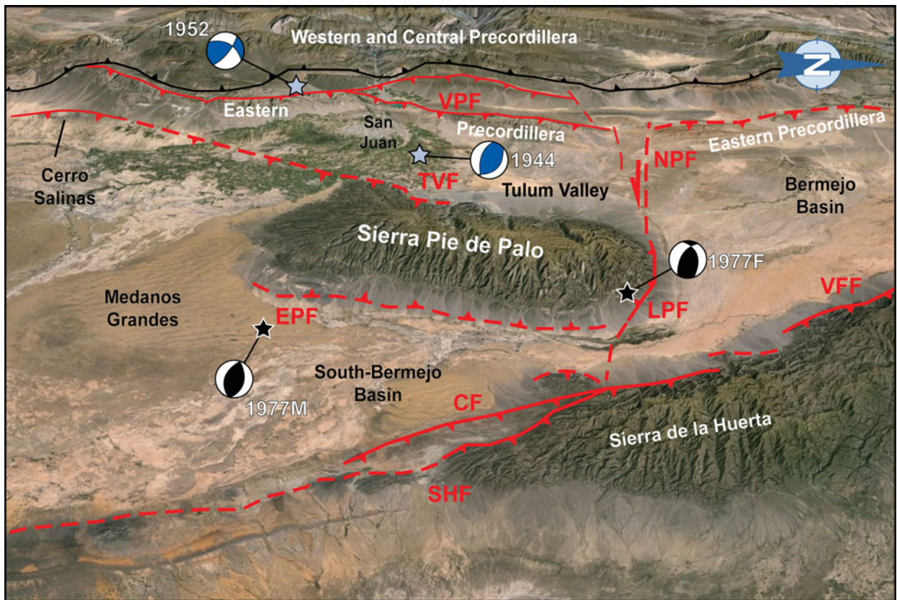
Figure 2. (Colour online) Tentative schematic structural map of the Sierra Pie de Palo and surroundings showing the major faults. Modified after Siame et al. (2015). CF, Las Chacras Fault; EPF, East Pie de Palo Fault; LPF, Los Pajaritos Fault; NPF, North Pie de Palo Fault; SHF, Sierra de la Huerta Fault; TVF, Tulum Valley Fault; VFF, Valle Fértil Fault; VPF, Villicum–Pedernal Fault. The dashed line east of the Pie de Palo is the limit between alluvial fans and the flat playa type of Quaternary sediments. Its linear geometry suggests that the alluvial fans are slightly tilted; this should be controlled by the blind E-verging thrust. Indeed, the older fan surfaces are steeper than the younger ones (the older the fan, the steeper its surface). Light blue stars locate 1944 ( M_w = 7.0 ) and 1952 ( M_w = 6.8 ) earthquakes with focal mechanism solutions after Alvarado and Beck (2006). Black stars locate fore- and main shocks of the Cauçete 1977 ( M_s = 7.4 ) earthquake (focal mechanism solutions after Langer & Hartzell, 1996).
