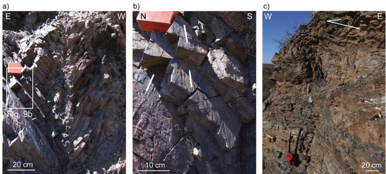
Figure 9. (Colour online) Field photographs of folds affecting the basement rocks. (a) Fold with sharp and fractured hinge and (b) associated foliation-parallel slip (site 2, Fig. 5). Fold and slip indicate an E–W shortening. (c) Larger-scale fold in the basement. Note the W-verging kinematics.
