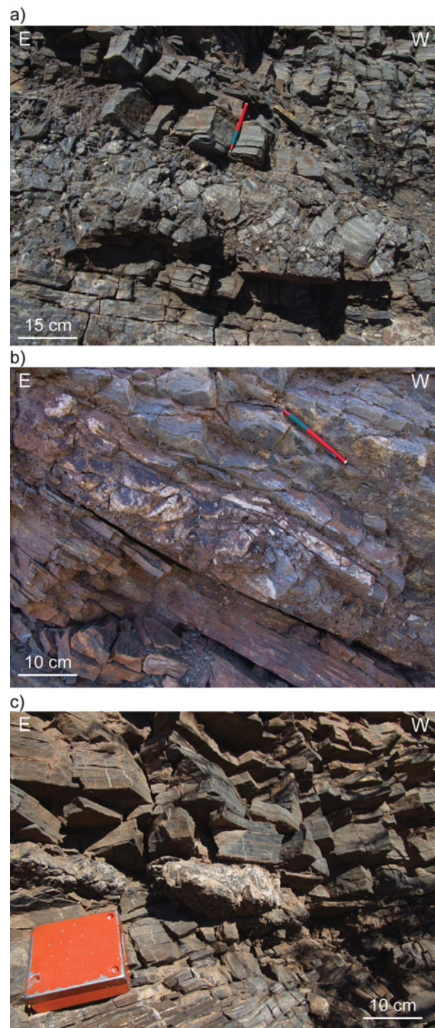
Figure 10. (Colour online) Foliation-parallel breccias. (a) With no cement (site 23, Fig. 5). (b, c) With more cement (site 10, Fig. 5).
