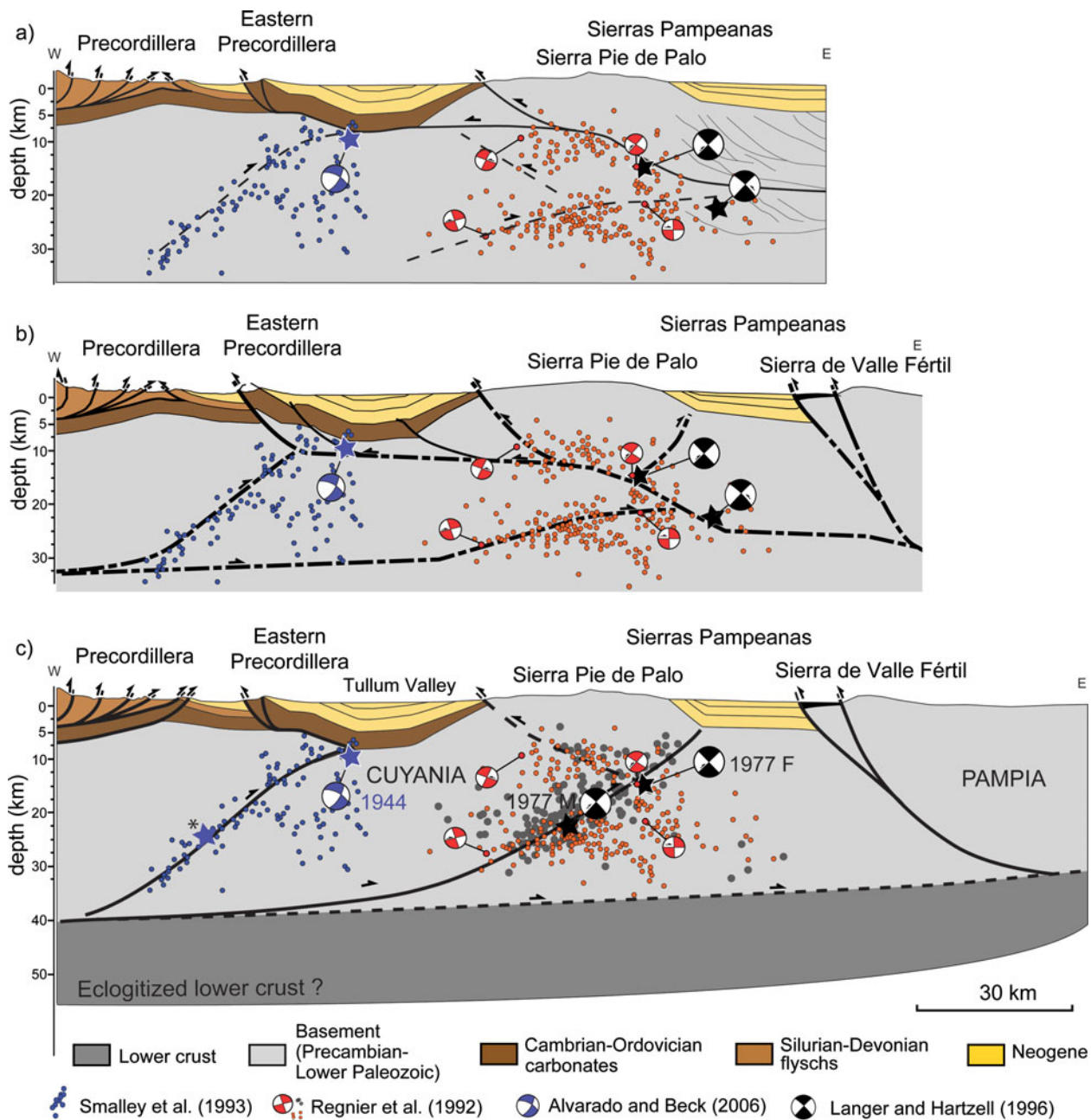
Figure 14. (Colour online) Crustal-scale cross-section of the Sierra Pie de Palo, the Sierra Valle Fértil and the Precordillera (see Fig. 1b for location). (a) From Vergés et al. (2007); (b) in Siame et al. (2015); and (c) this study. In (c), the front of the Precordillera has been modified after Alonso et al. (2014). The asterisk near the star along the western crustal E-verging thrust represents an alternative solution for the 1944 focus (from Meigs and Nabelek, 2010). The 1977M earthquake focus have been translated 30 km to the west as suggested in Regnier et al. (1992).
