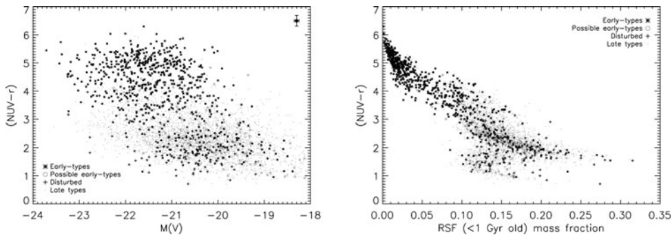
Figure 1. LEFT-HAND PANEL: Rest-frame ( NUV - r ) colour-magnitude relation of the E-CDFS galaxy population. RIGHT-HAND PANEL: Rest-frame ( NUV - r ) colour plotted against the RSF in the E-CDFS galaxy population. The NUV ( \sim 2300\text{\AA} ) and r band filters are taken from the GALEX and SDSS filtersets respectively.
