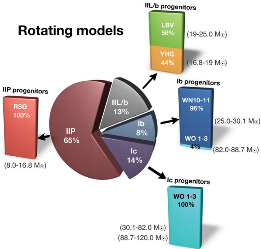
Figure 1. Diagram illustrating, for different core-collapse SN types, their relative rates and the types of progenitors and their respective frequencies. Initial mass ranges (indicated in parenthesis) and SN types are based on the criteria outlined in Georgy et al. (2012), assuming that the minimum amount of He in the ejecta to produce a SN Ib is 0.6 M_{\odot} .
