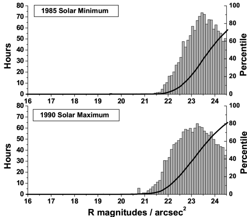
Figure 7 Intensity of the 630.0-nm [OI] line observed at the South Pole, in R magnitudes per square arcsecond. The left axis shows the number of hours per winter that a particular intensity is observed. The cumulative probability is shown on the right-hand axis.
