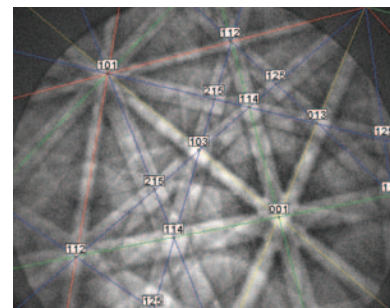
Top: Cartridge Brass, tint etched with Klemm's III, in crossed polarized light with a sensitive tint filter. 50x. Bottom: Cartridge Brass indexed EBSD pattern. Quality Index: 221±8.6
