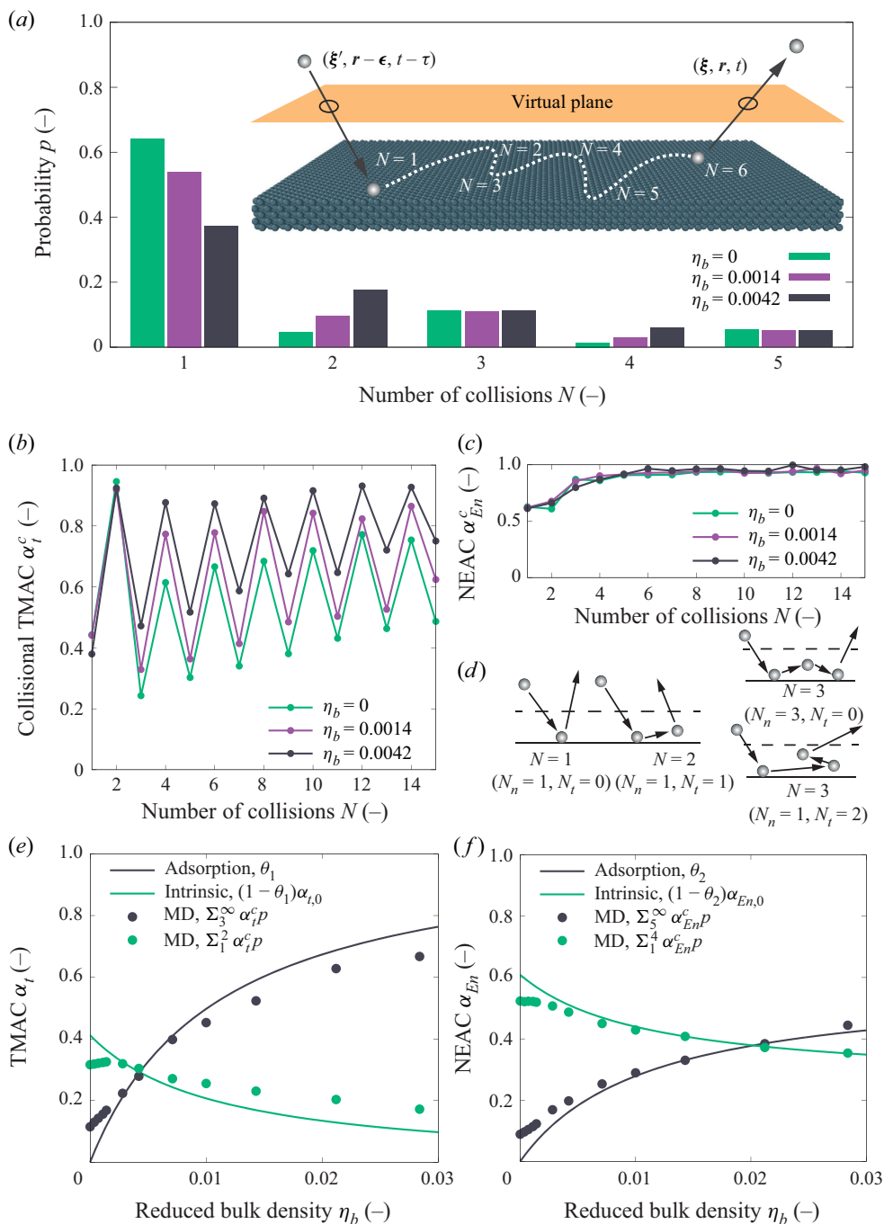
Figure 2. Scattering process of argon molecules on a platinum surface at 423 K. (a) Probability histogram of the number of collisions, with the inset indicating the tracking of the scattering process. (b) TMAC vs number of collisions. (c) NEAC vs number of collisions. (d) Qualitative schematics of odd vs even collisions. Contributions to (e) TMAC and (f) NEAC of molecules suffering two, for TMAC, and up to four, for NEAC, collisions (green colour) and multiple collisions (black colour) as functions of the reduced bulk density. Solid symbols are MD results and solid lines are the predictions of our calibrated SK, (3.3).
