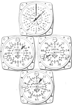
A typical layout of Decca Decometers including the new Lane Identification differential meter.
