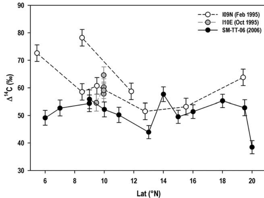
Figure 2 Spatial variation of \Delta^{14}\text{C} in the DIC of the surface Bay of Bengal during the WOCE expedition and this study.
