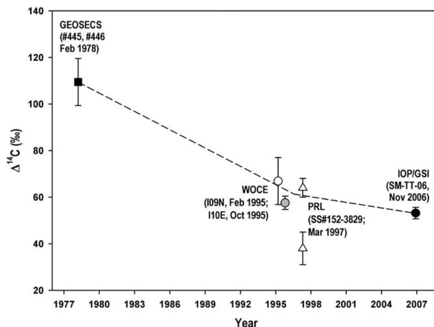
Figure 3 Decadal \Delta^{14}\text{C} changes in the DIC of the surface Bay of Bengal (near 10^\circ\text{N} , 86^\circ\text{E} )
