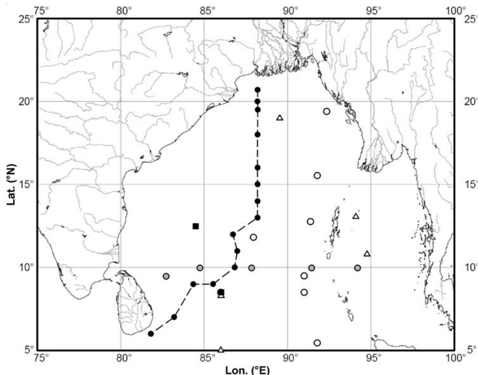
Figure 1 ^{14}\text{C} sampling stations in the Bay of Bengal: GEOSECS (stations #445 and #446, squares); WOCE (I09N, open circles; I10E, shaded circles); PRL (triangles); SM-TT-06 cruise (filled circles).
