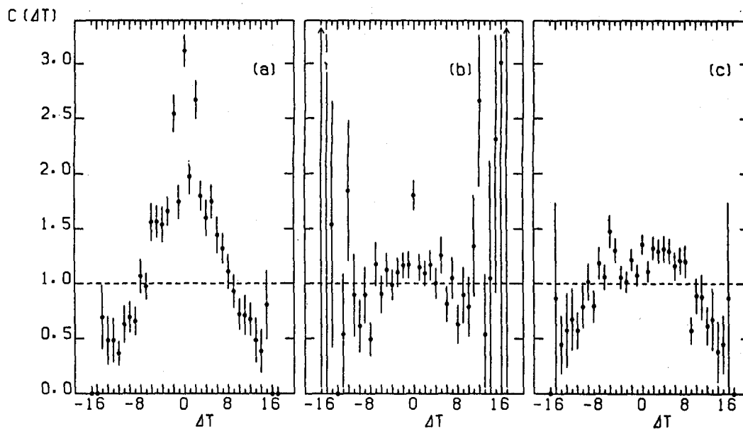
Fig 3. The morphological type correlation spectrum C(\Delta T) for various sub-samples. (a) For the pairs of both non-IRAS galaxies. (b) For the pairs of both IRAS galaxies. (c) For the pairs of IRAS galaxy and non-IRAS galaxy.
