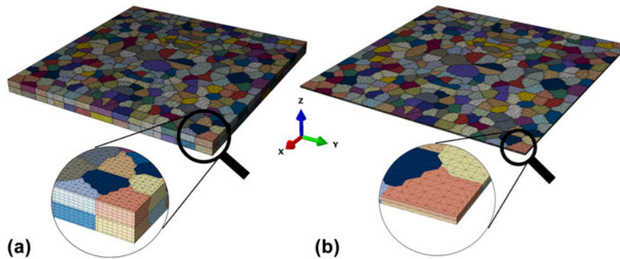
FIG. 7. The CPFE model meshes for the (a) 50–50 nm Mg/Nb composite and (b) 5–5 nm composite. Each model contains one layer each of Mg and Nb. Bottom images show zoomed-in view of the microstructures indicating different grain aspect ratios.
