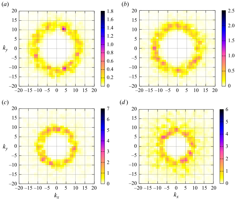
Figure 1. Surfaces of |a_k|^2 \times 10^8 in the condensate region for four simulations of Koročevič (2023) corresponding to four different mean wave slopes \mu , for (a) \mu = 0.054 , (b) \mu = 0.067 , (c) \mu = 0.093 , (d) \mu = 0.135 .
