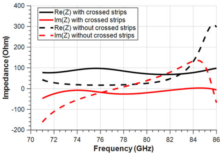
Figure 8. Simulated input impedance with and without crossed strips.
