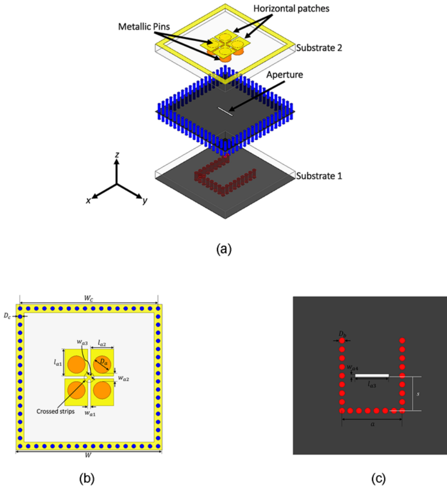
Figure 7. Geometry of the SIW-fed aperture-coupled ME dipole antenna: (a) dissection view, (b) top view of Substrate 2, and (c) top view of Substrate 1.
