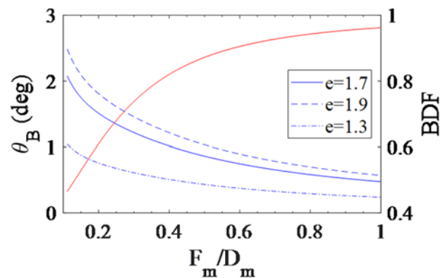
Figure 3. Lateral feed displacement effects as a function of F/D : red: BDF; blue: \theta_B for \delta_c = 2 cm and for different values of the subreflector eccentricity; e , at 77 GHz.
