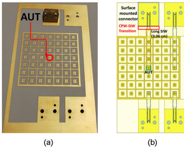
Figure 10. Proposed ME dipole in a 7 \times 7 feed array configuration: (a) photograph of the prototype and (b) layout of the array board.
