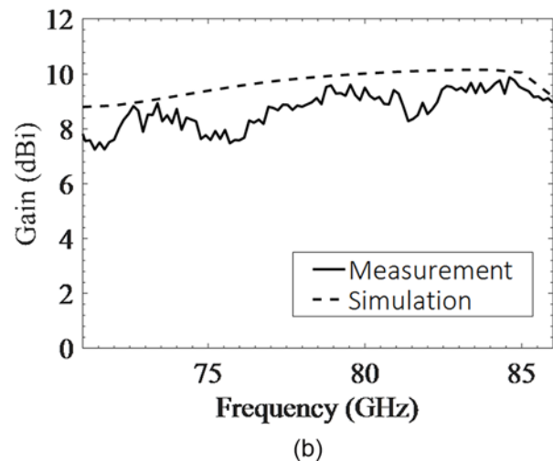
Figure 11. Simulated (dashed) and measured (solid) reflection coefficient (a) and gain (b) of the proposed SIW-fed aperture-coupled ME dipole. The radiating element taken as a reference is the central one.
