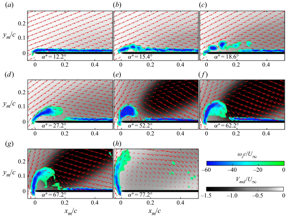
Figure 18. Progressive development of the normalised spanwise vorticity \omega_z c / U_\infty superimposed on the velocity vectors and estimated downwash V_{md} at the mid-span of the very low AR wing pitching at K = 0.08 as a function of \alpha^* .
