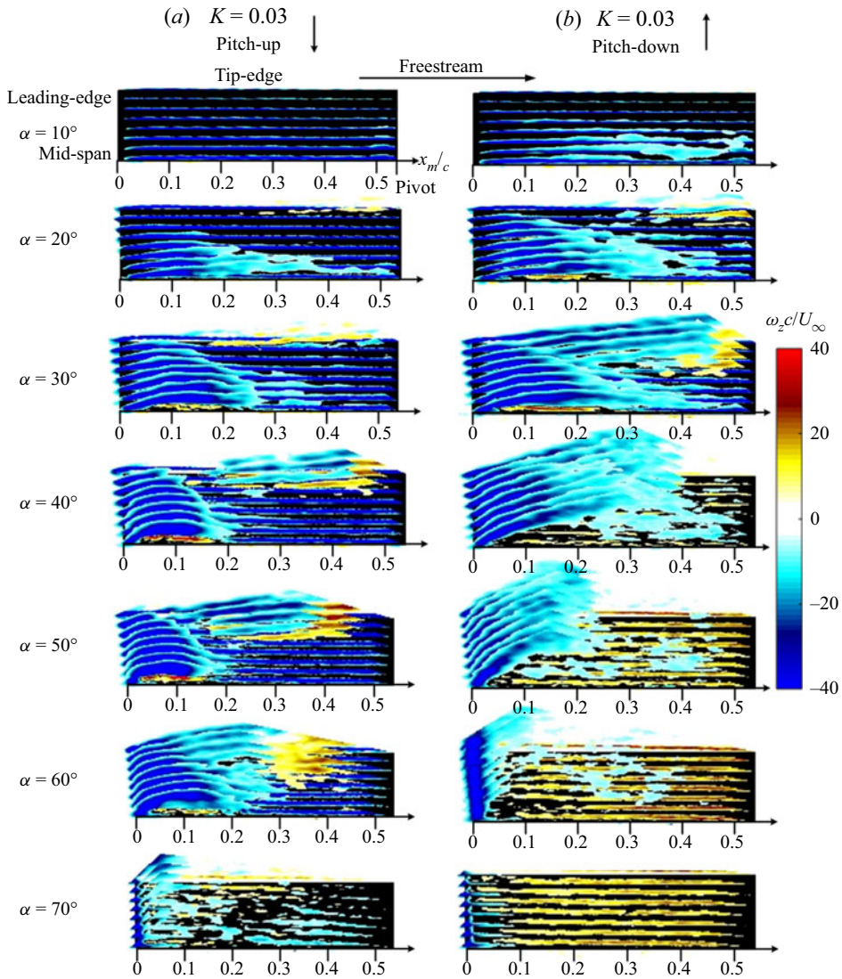
Figure 17. The phase-averaged normalised spanwise vorticity ( \omega_z c/U_\infty ) along the span vs AoA for the pitch-up and pitch-down wing at K = 0.03 . The colour bar on the right side applies to all plots.
