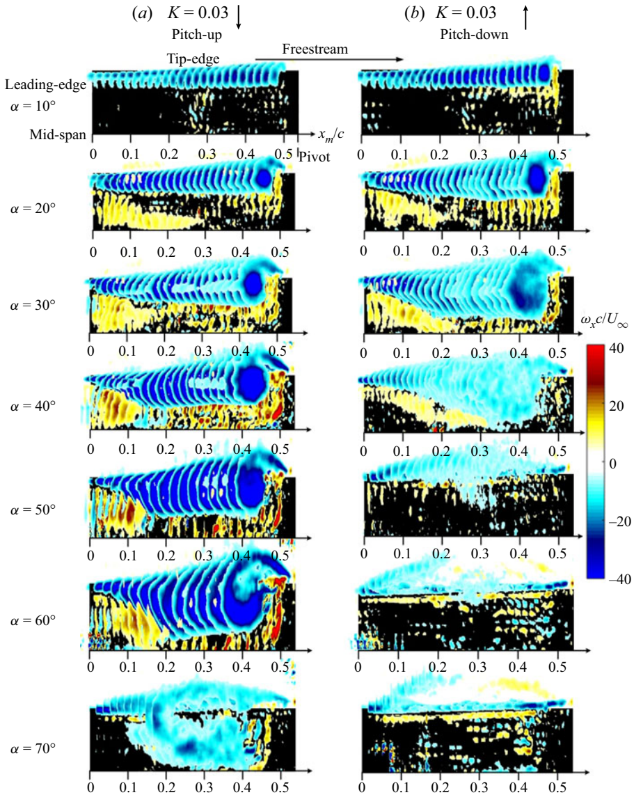
Figure 7. The phase-averaged normalized streamwise vorticity ( \omega_x c / U_\infty ) along the chord vs AoA for the wing pitching up and down at K = 0.03 . The colour bar on the right side applies to all plots.
