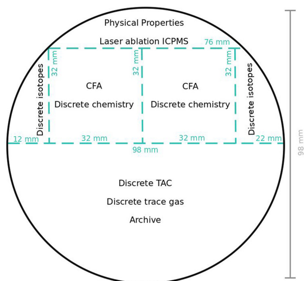
Fig. 2. Schematic of WACSWAIN ice core cross-sectional cutting plan. Dashed lines show lengthwise cuts.
