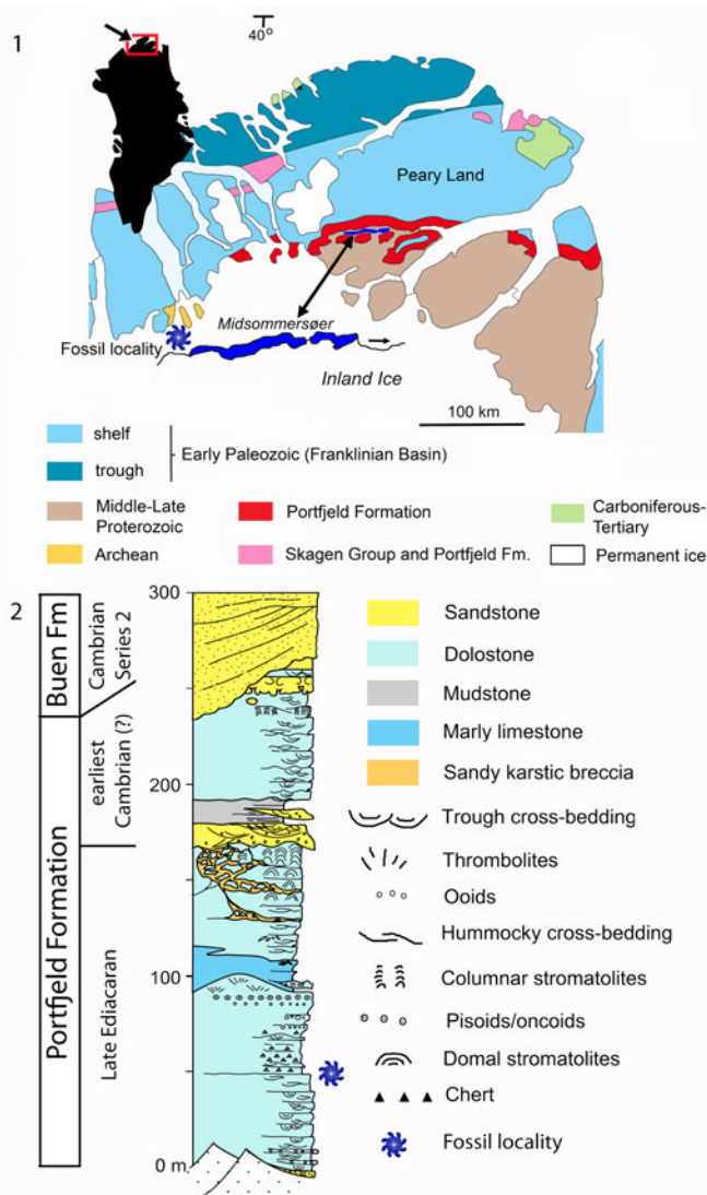
Figure 1. Simplified geological map and lithostratigraphic column of the Portfjeld Formation. (1) Geological map showing the sampling site at the western end of Midsommørsøer in North Greenland; (2) lithostratigraphic column through the Portfjeld Formation at eastern Midsommørsøer where the fossiliferous horizon is located at a lower level than in the fossil locality at western Midsommørsøer (see discussion in text; modified from Willman et al., 2020).
