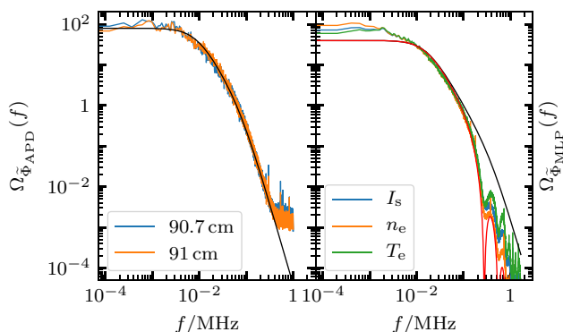
FIGURE 8. Left: PSD of the GPI data from two different radial positions measured in discharge 3 and (2.4) using parameters from a least-squares fit. Right: PSDs of the MLP signals and both (2.5) (red line) and (2.4) (black line) evaluated using parameters found from a least-squares fit.
