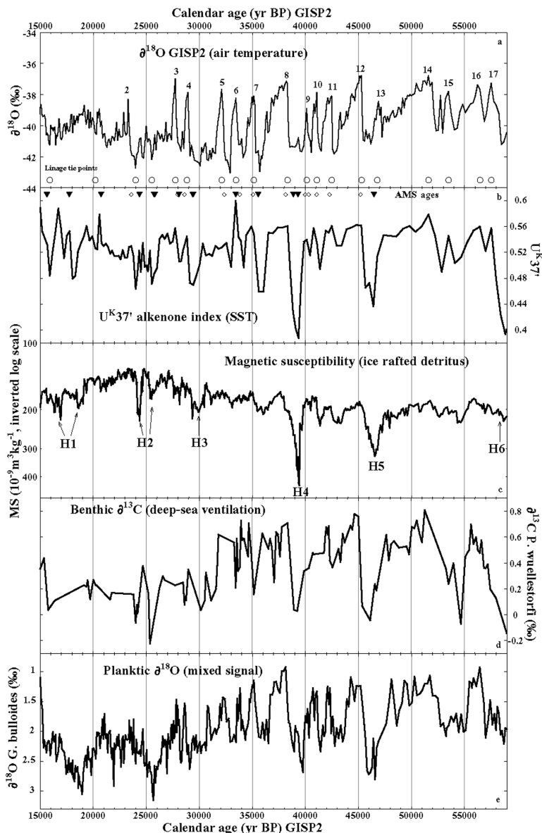
Figure 4 Time series of climatic and oceanographic variations in Greenland and the Iberian Margin during the last 59,000 yr before AD 1950: (a) \delta^{18}\text{O} measured in the Greenland Summit GISP2 core (Stuiver and Grootes 2000). The data set and its time scale were extracted from the file gispd18o.dat in the CD-ROM compiled by Cross (1997) distributed jointly by the World Data Center for Paleoclimatology at NOAA-NGDC and the Institute of Arctic and Alpine Research. Numbers depict the Dansgaard-Oeschger events following Dansgaard et al. (1993). Small open circles represent the tie points used for the correlation with the deep-sea core U_{37}^{K'} index (Figure 4b); (b–e): stratigraphy of core MD952042 along a time scale tuned to the curve in (a) by means of the Linage software (Paillard et al. 1996); (b) U_{37}^{K'} alkenone index a proxy for sea-surface temperature (SST); raw data from Pailler and Bard 2002). Symbols locate the samples used for AMS dating (black triangles are data from NOSAMS [Bard et al. 2004a,b]; open diamonds are the data from GifA and Kiel [Shackleton et al. 2004]); (c) magnetic specific susceptibility record plotted on an inverted log scale (raw data from Thouveny et al. 2000). Maximum values (i.e. troughs in the curve) are used to identify the ice-rafted detritus injected during Heinrich and other events. The numbers represent the 6 classical Heinrich events. Off the Iberian Margin, these events (e.g. H1 and H2) often contain 2 peaks which can be seen both on (b) and (c) (see discussion in Thouveny et al. 2000; and Bard et al. 2000 and references therein); (d) \delta^{13}\text{C} measured on benthic foraminifera and used as a proxy for the ventilation of the deep Atlantic (raw data from Shackleton et al. 2000); (e) \delta^{18}\text{O} values for planktonic foraminifera (raw data from Cayre et al. 1999; Shackleton et al. 2000).
