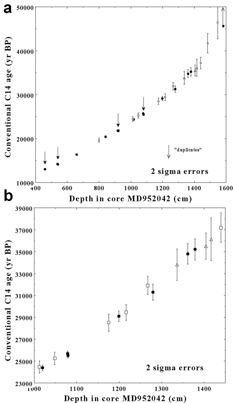
Figure 3 ^{14}\text{C} ages from Table 2 plotted versus depth in core MD952042: (a) data between 400 and 1600 cm; (b) expanded view of the data between 1000 and 1450 cm. Black dots are samples dated at NOSAMS (Bard et al. 2004a,b); open squares and triangles are data from GifA and Kiel, respectively (Shackleton et al. 2004). Downward arrows indicate depths for which “duplicate” measurements were performed at NOSAMS (see text for more details). All ^{14}\text{C} errors are quoted at the 2- \sigma level. An upward arrow has been used for the lower-bound ^{14}\text{C} age obtained for the 1581.5-cm section (see Table 2).
