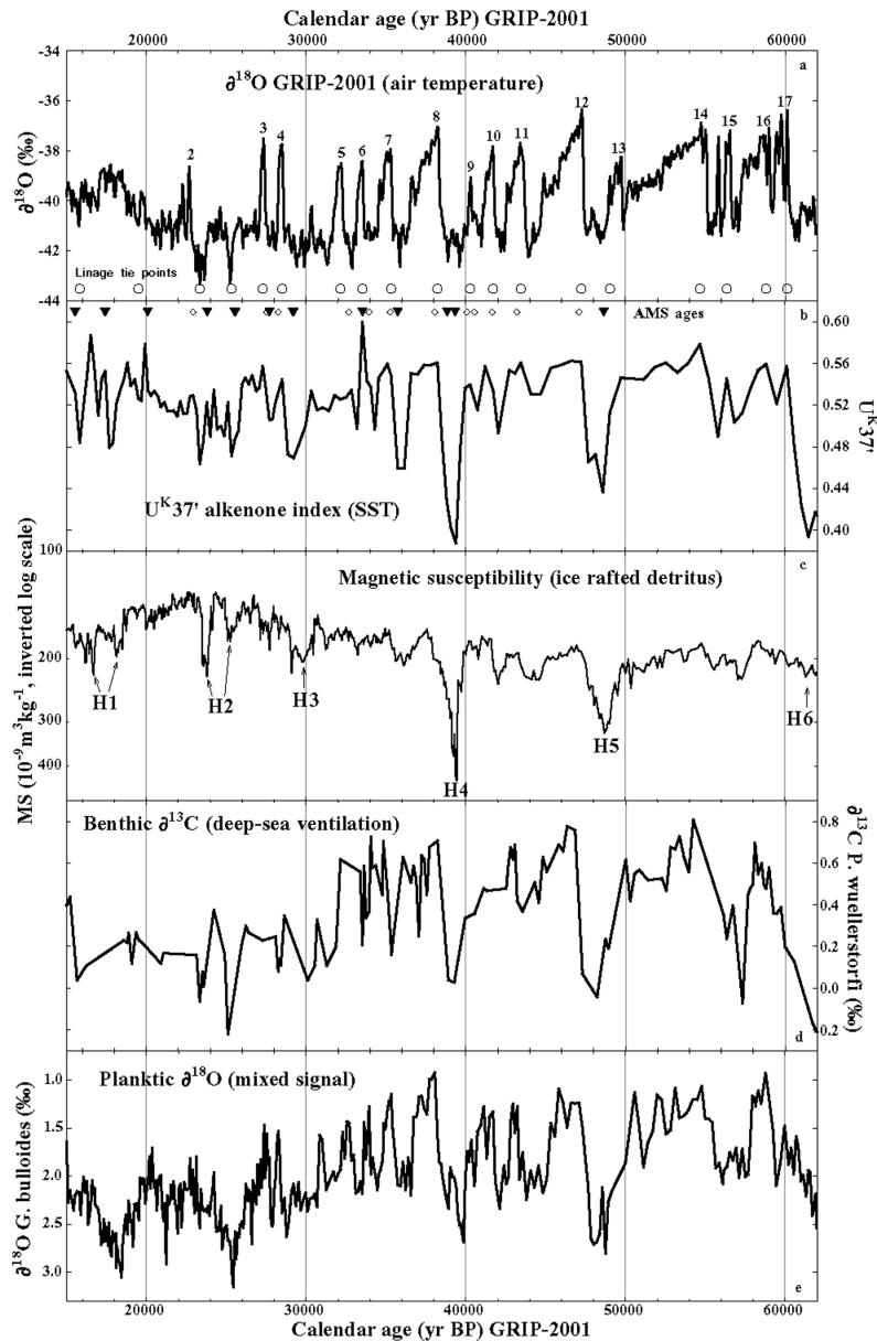
Figure 5 Time series of climatic and oceanographic variations in Greenland and the Iberian Margin during the last 62,000 yr before AD 1950: (a) \delta^{18}\text{O} measured in the Greenland Summit GRIP core (Dansgaard et al. 1993; Johnsen et al. 2001). The time scale is from Johnsen et al. (2001). Numbers depict the Dansgaard-Oeschger events following Dansgaard et al. (1993). Small open circles represent the tie points used for the correlation with the deep-sea core U_{37}^K index (Figure 5b). These tie points are the same as those used for the matching with GISP2 (minor update with respect to Bard et al. 2004a,b, which is responsible for small differences in the calendar age estimates listed in Table 2). (b–e): stratigraphy of core MD952042 along a time scale tuned to the curve in (a) by means of the Linage software (Paillard et al. 1996); (b) U_{37}^K alkenone index, a proxy for sea-surface temperature (SST; raw data from Pailler and Bard 2002). Symbols locate the samples used for AMS dating (black triangles are data from NOSAMS [Bard et al. 2004a,b]; open diamonds the data from GifA and Kiel [Shackleton et al. 2004]); (c) magnetic specific susceptibility record plotted on an inverted log scale (raw data from Thouveny et al. 2000). Maximum values (i.e. troughs in the curve) are used to identify the ice-rafted detritus injected during Heinrich and other events. The numbers represent the 6 classical Heinrich events. Off the Iberian Margin, these events (e.g. H1 and H2) often contain 2 peaks which can be seen both on (b) and (c) (see discussion in Thouveny et al. 2000; and Bard et al. 2000 and references therein); (d) \delta^{13}\text{C} measured on benthic foraminifera and used as a proxy for the ventilation of the deep Atlantic (raw data from Shackleton et al. 2000); (e) \delta^{18}\text{O} values for planktonic foraminifera (raw data from Cayre et al. 1999; Shackleton et al. 2000).
