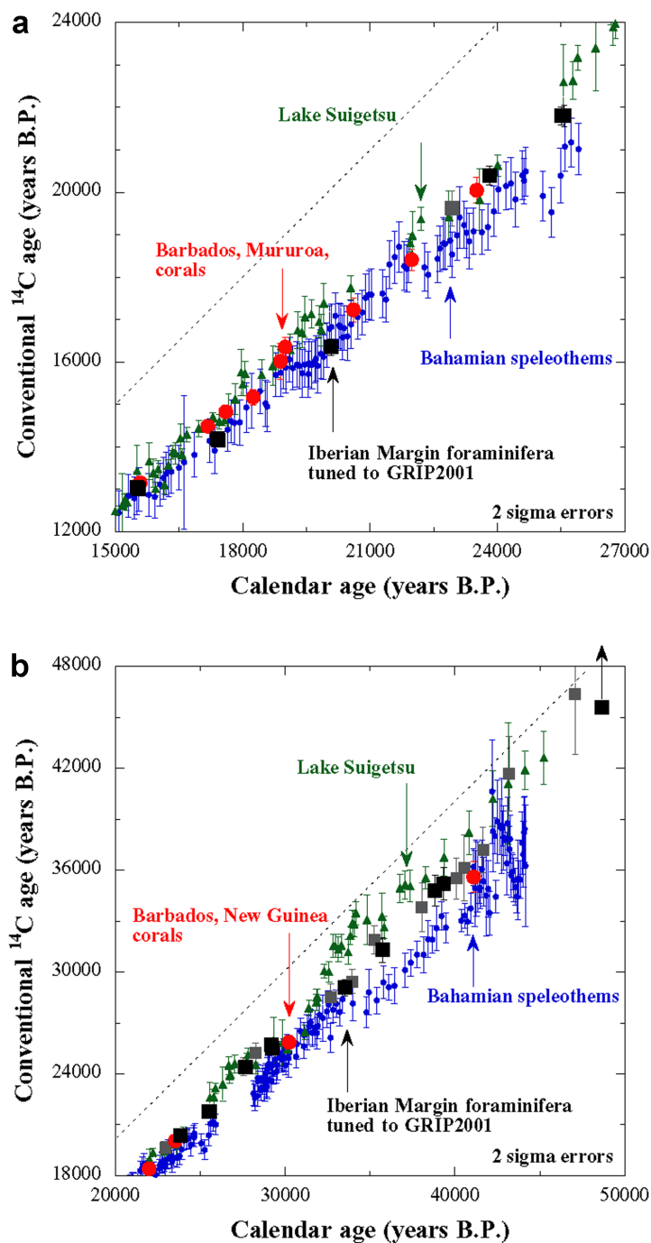
Figure 7 ^{14}\text{C} ages plotted versus calendar ages: (a) data within the range of IntCal98 in the interval between 15,000 and 24,000 cal BP; (b) data beyond the range of IntCal98 (Stuiver et al. 1998). Squares show the data based on ^{14}\text{C} data of the Iberian Margin sediments tuned to GRIP. Black symbols are data from NOSAMS (Bard et al. 2004a,b); gray symbols are the data from GifA and Kiel (Shackleton et al. 2004). Red dots represent data from Barbados, Mururoa, and New Guinea corals (Bard et al. 1998); green triangles = Lake Suigetsu varves (Kitagawa and van der Plicht 1998, 2000); and blue dots = Bahamian speleothems (Beck et al. 2001). All ^{14}\text{C} errors are quoted at the 2- \sigma level. An arrow has been used for the lower-bound ^{14}\text{C} age obtained for the 1581.5-cm section (see Table 2).
