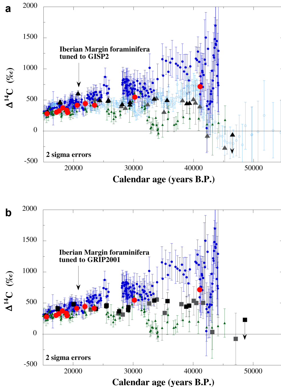
Figure 8 Atmospheric \Delta^{14}\text{C} versus time as calculated using the AMS- ^{14}\text{C} ages plotted in Figures 6 and 7. Triangles and squares show the data based on ^{14}\text{C} data of the Iberian Margin sediments tuned to GISP2 (a) and GRIP (b), respectively. Black symbols are data from NOSAMS (Bard et al. 2004a,b); gray symbols are the data from GifA and Kiel (Shackleton et al. 2004). Red dots represent data from Barbados, Mururoa, and New Guinea corals (Bard et al. 1998); green triangles = Lake Suigetsu varves (Kitagawa and van der Plicht 1998, 2000); blue dots = Bahamian speleothems (Beck et al. 2001); and open blue circles = Cariaco Basin ODP Core (Hughen et al. 2004). All ^{14}\text{C} errors are quoted at the 2- \sigma level. An arrow has been used for the higher-bound \Delta^{14}\text{C} age obtained for the 1581.5-cm section (see Table 2).
