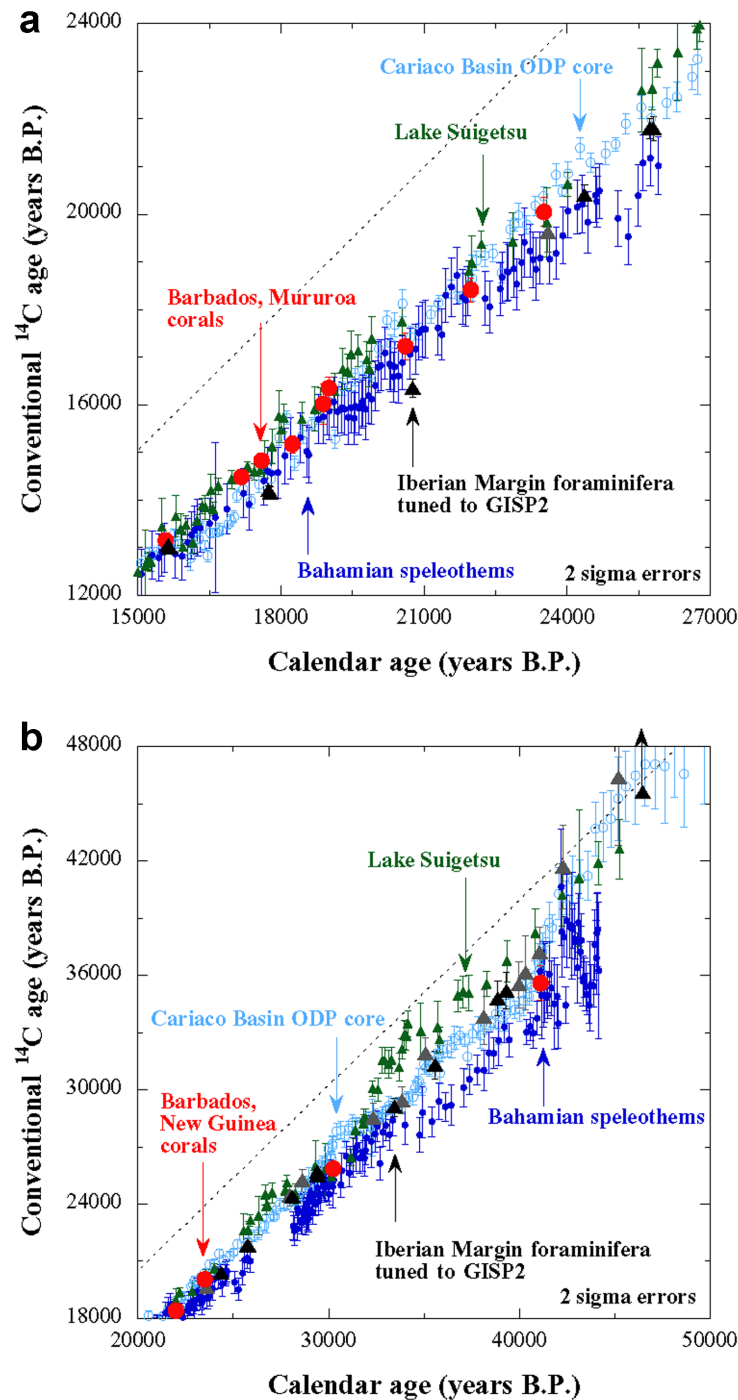
Figure 6 ^{14}\text{C} ages plotted versus calendar ages: (a) data within the range of IntCal98 in the interval between 15,000 and 24,000 cal BP; (b) data beyond the range of IntCal98 (Stuiver et al. 1998). Triangles show the data based on ^{14}\text{C} data of the Iberian Margin sediments tuned to GISP2. Black symbols are data from NOSAMS (Bard et al. 2004a,b); gray symbols are the data from GifA and Kiel (Shackleton et al. 2004). Red dots represent the IntCal98 data from Barbados, Mururoa, and New Guinea corals (Bard et al. 1998); green triangles = Lake Suigetsu varves (Kitagawa and van der Plicht 1998, 2000); blue dots = Bahamian speleothems (Beck et al. 2001); and open blue circles = Cariaco Basin ODP Core (Hughen et al. 2004). All ^{14}\text{C} errors are quoted at the 2- \sigma level. An arrow has been used for the lower-bound ^{14}\text{C} age obtained for the 1581.5-cm section (see Table 2).
