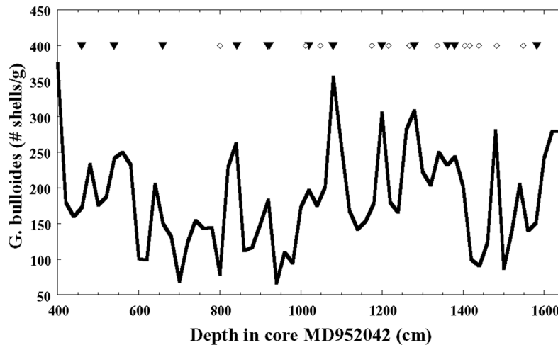
Figure 2 Abundances of Globigerina bulloides in core MD952042 expressed in terms of number of shells per gram of sediment (raw data from Cayre et al. 1999). Symbols represent the depths for which ^{14}\text{C} ages on monospecific samples were measured: black triangles (Bard et al. 2004a,b) and open diamonds (Shackleton et al. 2004). Note that the latter data set has an additional uncertainty linked to the fact that shells were not always sampled in abundance maxima observed for this species of foraminifera.
