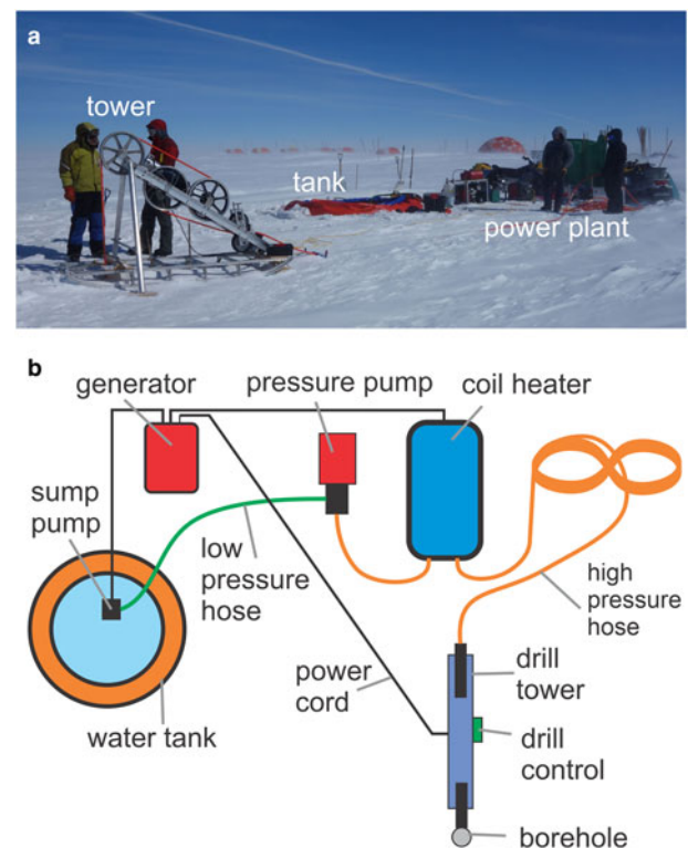
Fig. 1. Simple hot water drill for firn. (a) Photograph showing drill tower (left), water reservoir (center) and power plant (right); (b) schematic diagram showing components of the drill.
