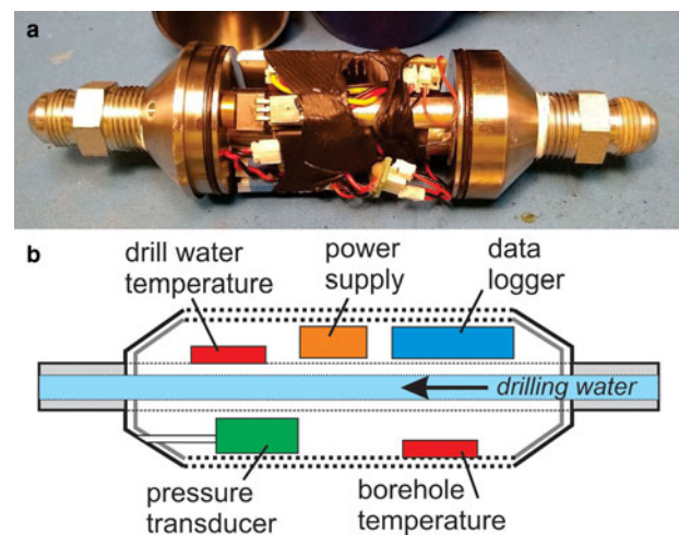
Fig. 2. Instrumented drill stem. The 5 cm diameter stainless steel pod has pressure couplings at both ends to allow mounting inline on the hose or stem. (a) Photograph showing stem with outer housing removed to show internals and sealing gaskets. (b) Generalized schematic diagram showing electronic components. Data logger includes clock and com port.
