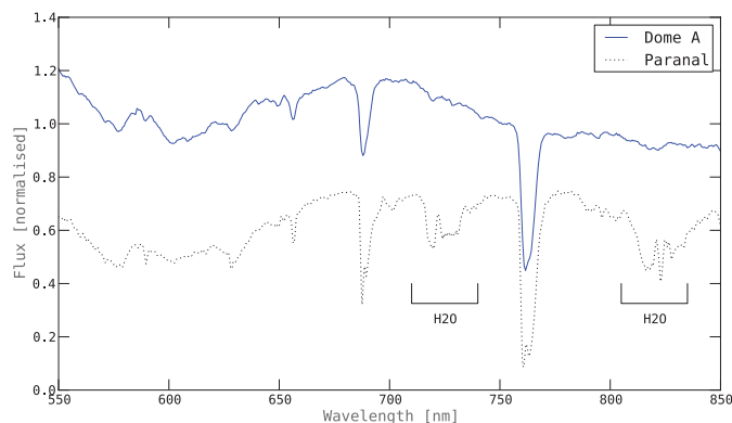
Figure 3. Comparison of Dome A and Paranal twilight sky spectra. The lack of H 2 O absorption in the Dome A spectrum is evident. Both spectra were obtained while the Sun was \sim 1.4^\circ below the horizon. The Dome A spectrum has been offset by +0.3. From Sims et al. (2012).
